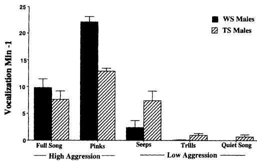
FIGURE 1. Mean ( \pm SE) vocalization rates of white-striped (WS, n = 19 ) and tan-striped (TS, n = 22 ) male White-throated Sparrows responding to simulated territorial intrusion.
